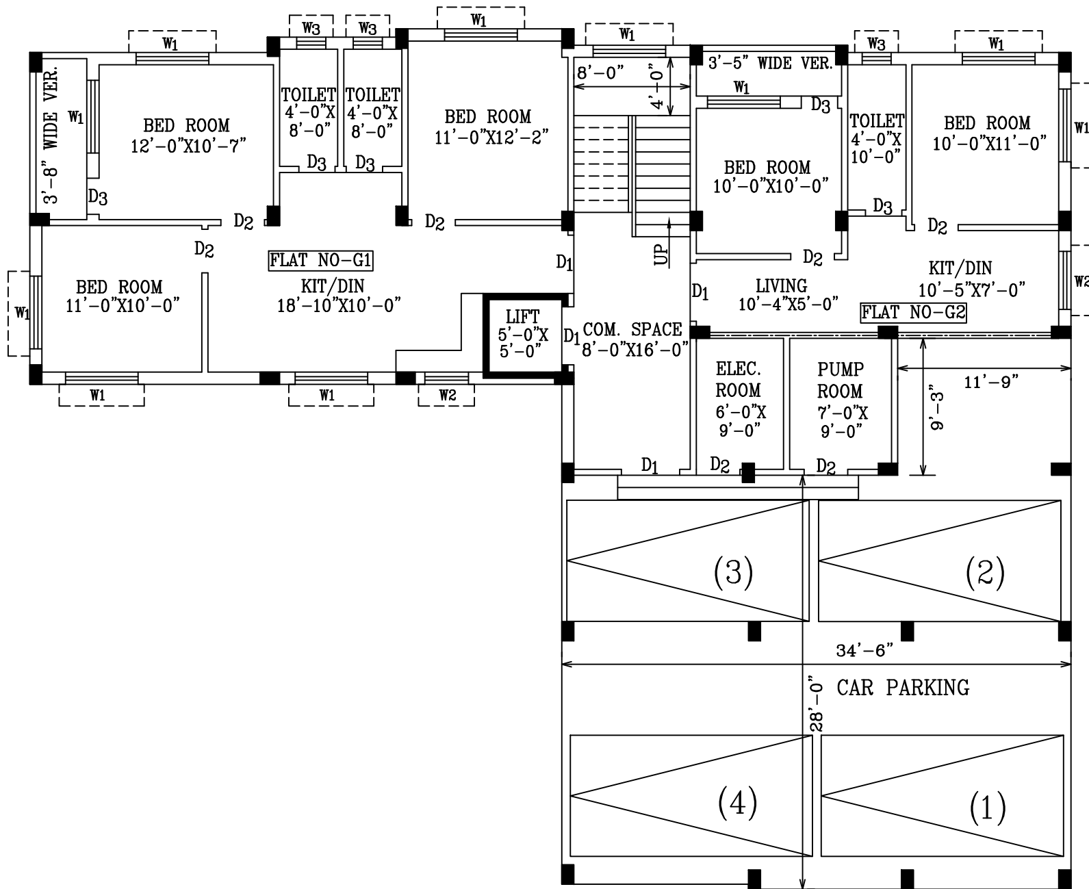
PROPOSED GROUND FLOOR PLAN SCALE- 1:100 BLOCK-C
